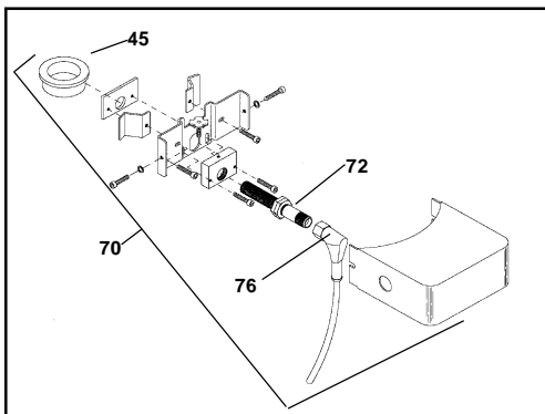
2" Bracket
