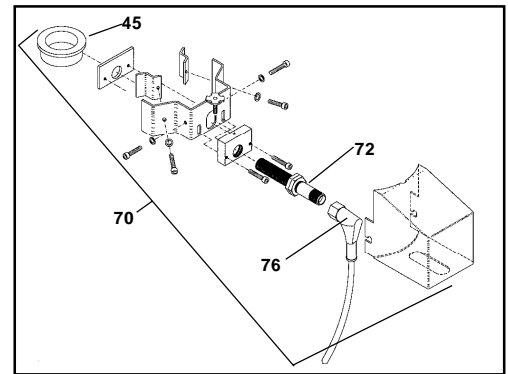
2.5" and 3" Bracket
